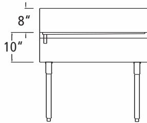
TYPICAL ELEVATION
